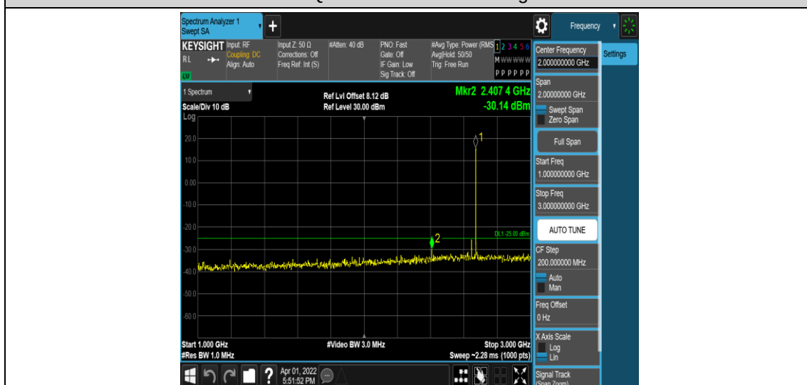
Band41-20MHz-16QAM-41490-1RB#0-Range4:1000~3000MHz
