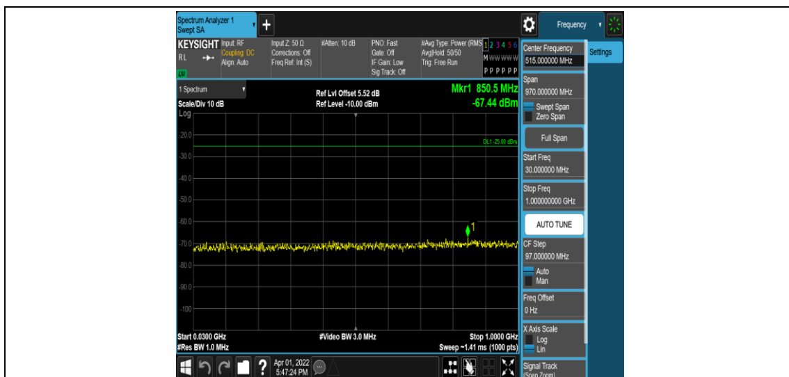
Band41-20MHz-16QAM-39750-1RB#0-Range3:30~1000MHz
