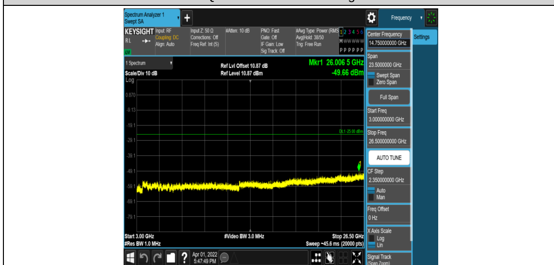
Band41-20MHz-16QAM-39750-1RB#0-Range5:3000~26500MHz
