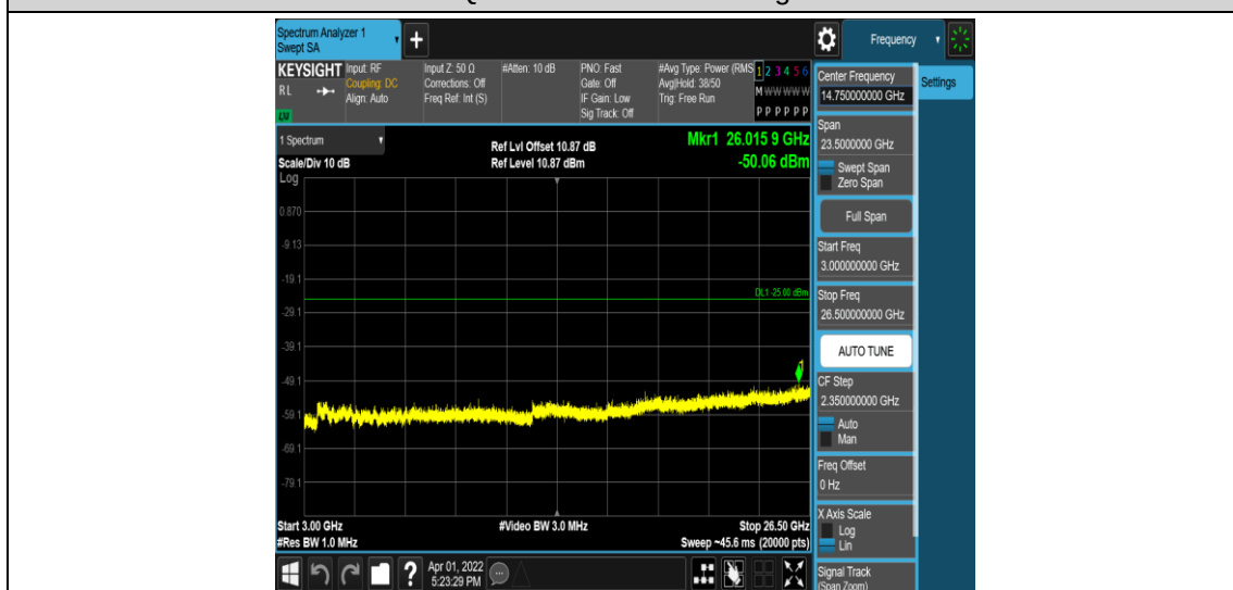
Band41-15MHz-16QAM-39725-1RB#0-Range5:3000~26500MHz
