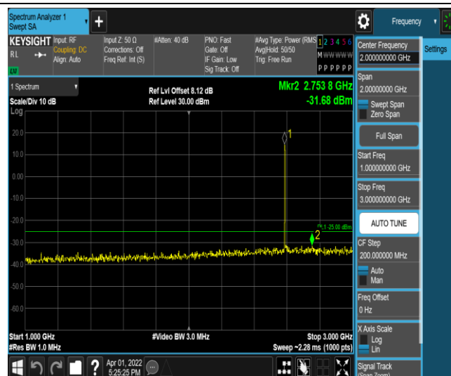
Band41-15MHz-16QAM-40620-1RB#0-Range4:1000~3000MHz
