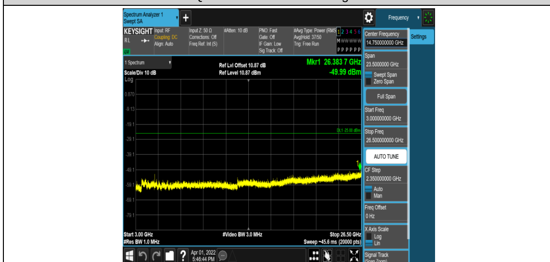
Band41-20MHz-QPSK-39750-1RB#0-Range5:3000~26500MHz
