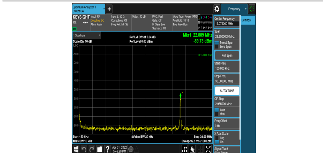
Band41-20MHz-16QAM-40620-1RB#0-Range2:0.15~30MHz
