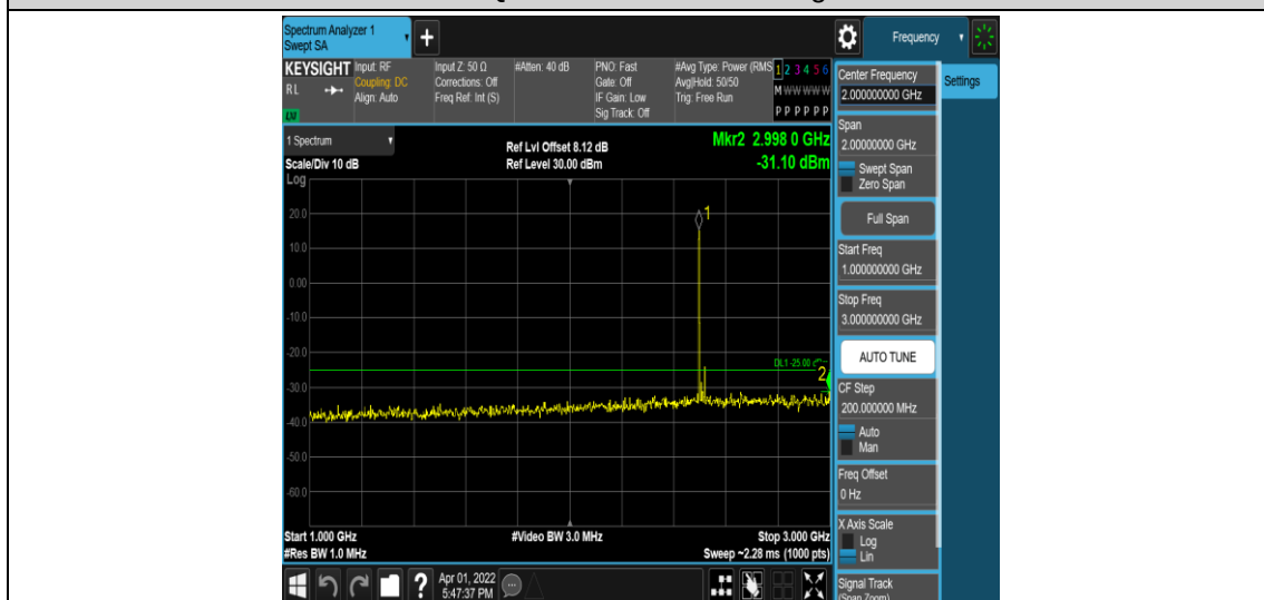
Band41-20MHz-16QAM-39750-1RB#0-Range4:1000~3000MHz
