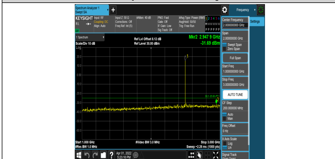
Band41-15MHz-16QAM-39725-1RB#0-Range4:1000~3000MHz
