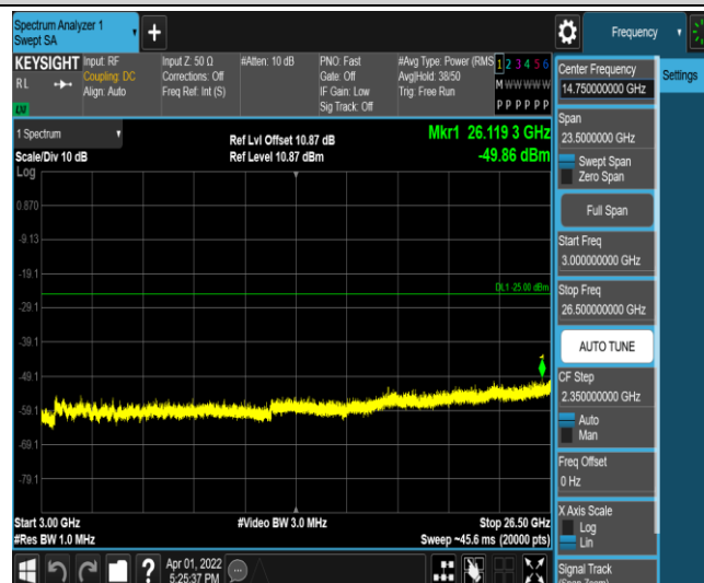
Band41-15MHz-16QAM-40620-1RB#0-Range5:3000~26500MHz
