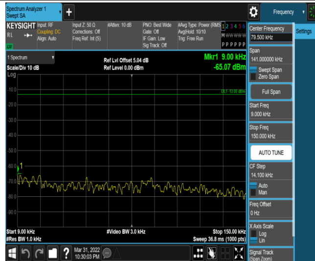
Band5-1.4MHz-16QAM-20643-1RB#0-Range1:0.009~0.15MHz
