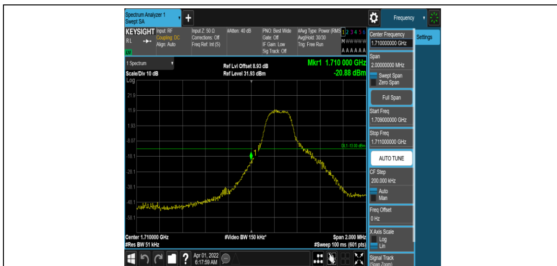
Band66-3MHz-16QAM-131987-1RB#0
