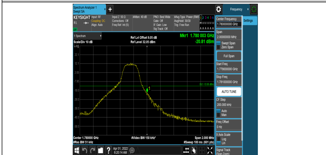
Band66-3MHz-16QAM-132657-1RB#14
