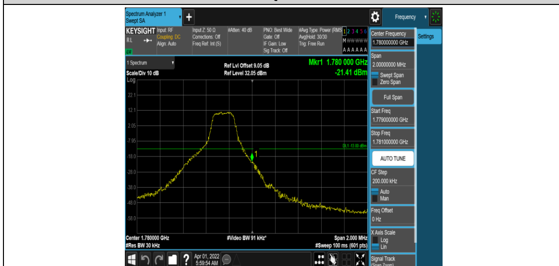
Band66-1.4MHz-QPSK-132665-1RB#5
