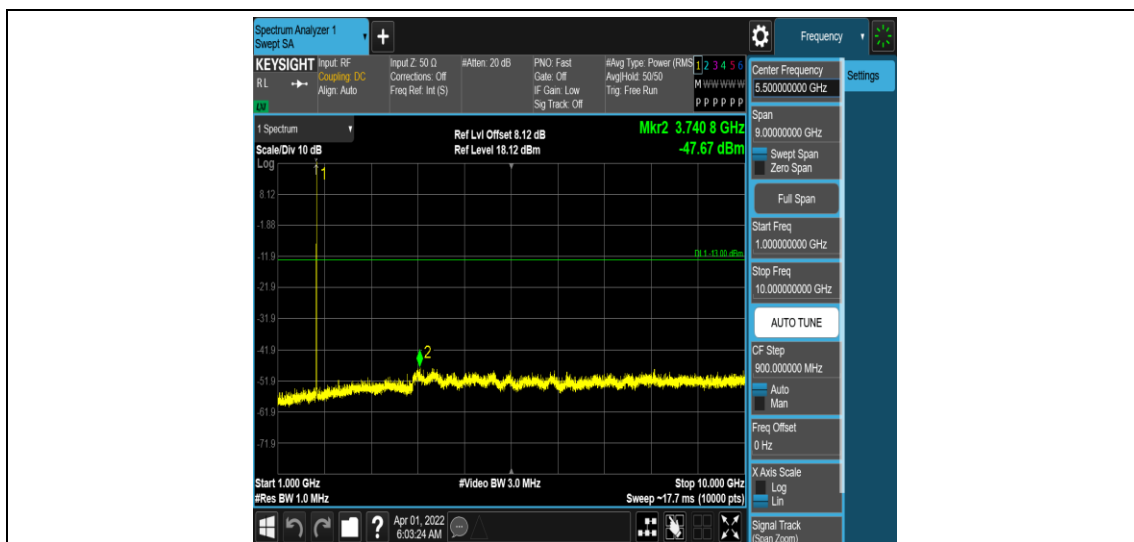
Band66-1.4MHz-QPSK-132322-1RB#0-Range4:1000~10000MHz
