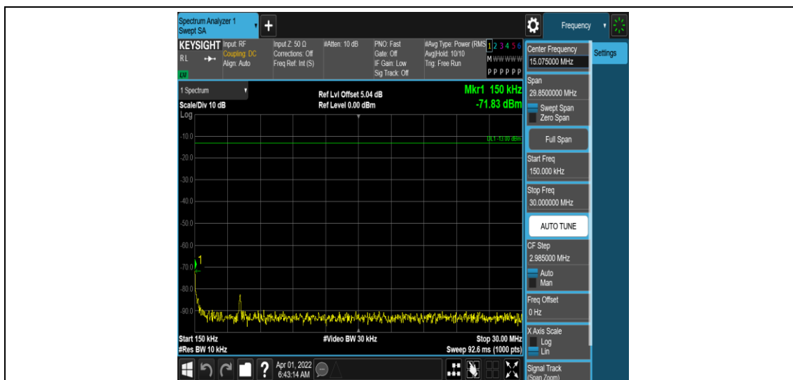
Band66-5MHz-16QAM-131997-1RB#0-Range2:0.15~30MHz
