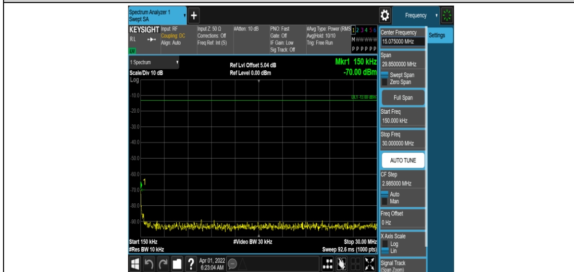
Band66-3MHz-QPSK-132322-1RB#0-Range2:0.15~30MHz
