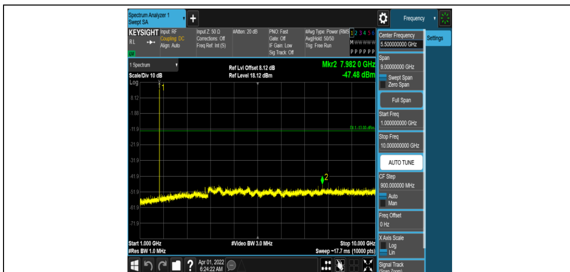
Band66-3MHz-16QAM-132322-1RB#0-Range4:1000~10000MHz
