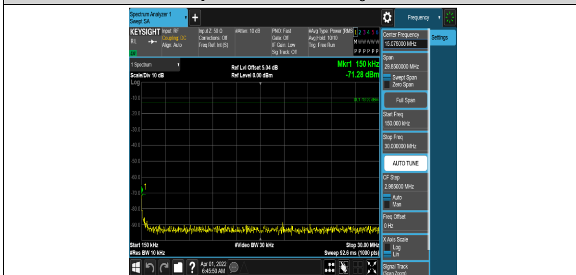
Band66-5MHz-QPSK-132647-1RB#0-Range2:0.15~30MHz
