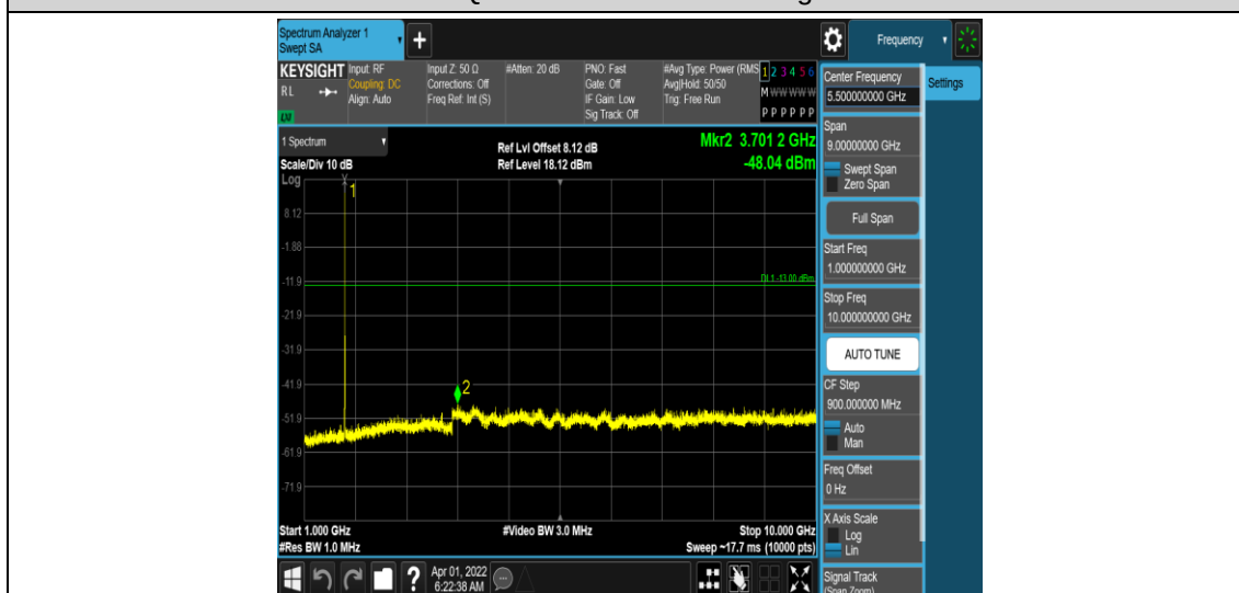
Band66-3MHz-16QAM-131987-1RB#0-Range4:1000~10000MHz
