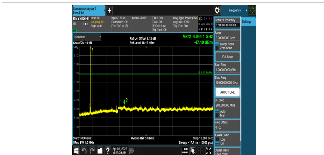
Band66-3MHz-QPSK-132322-1RB#0-Range4:1000~10000MHz
