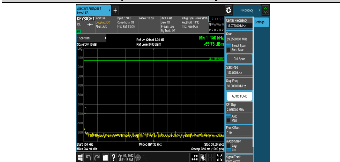
Band66-10MHz-QPSK-132622-1RB#0-Range2:0.15~30MHz
