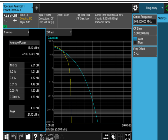
Band71-10MHz-16QAM-133172-1RB#0
