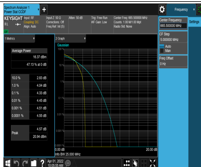
Band71-5MHz-16QAM-133147-1RB#0
