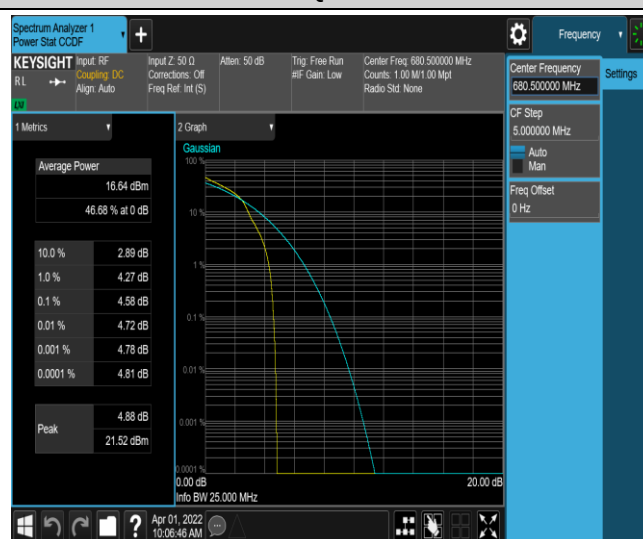
Band71-5MHz-16QAM-133297-1RB#0
