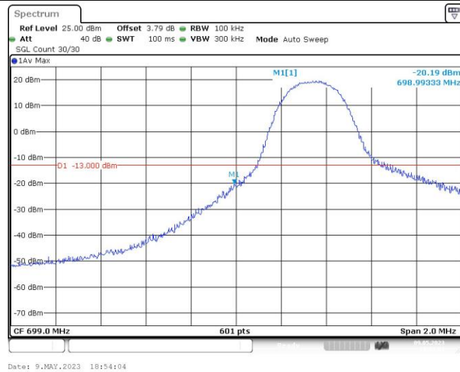
Band12-5MHz-QPSK-23035-1RB#24
