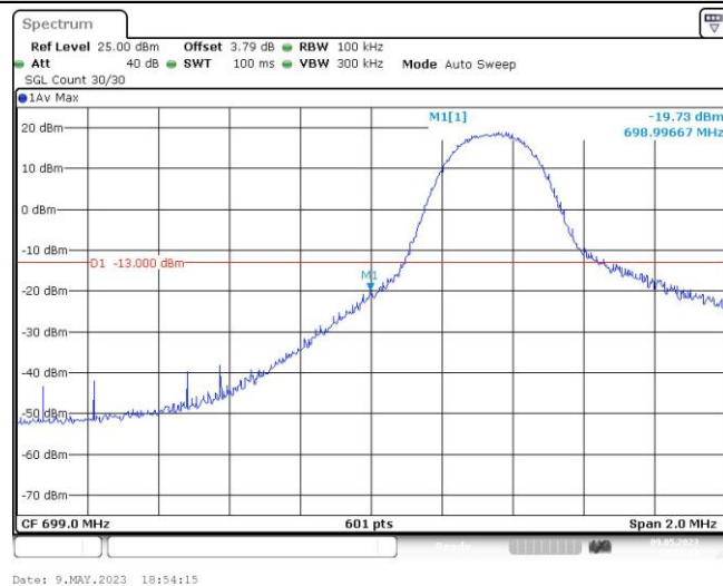
Band12-5MHz-16QAM-23035-1RB#24
