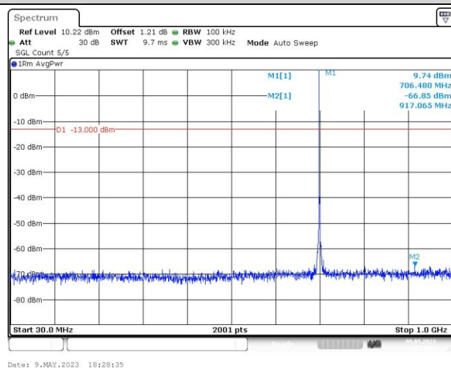
Band12-3MHz-16QAM-23095-1RB#0-Range4:1000~10000MHz
