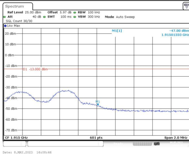
Band25-5MHz-QPSK-26665-1RB#24
