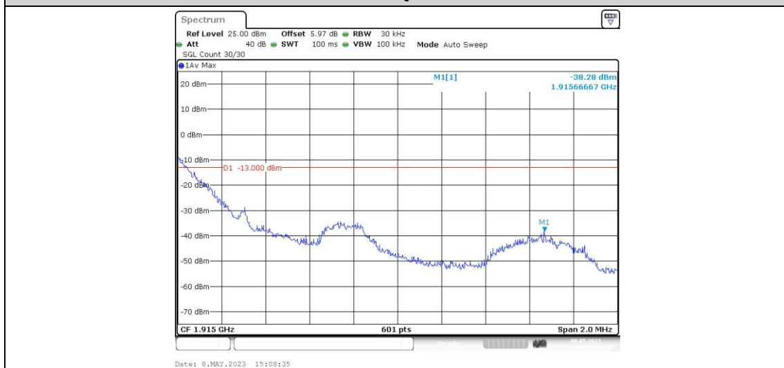
Band25-1.4MHz-16QAM-26683-1RB#5
