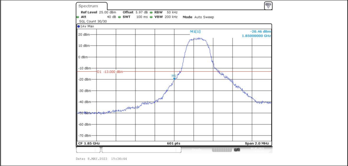
Band25-3MHz-QPSK-26055-1RB#14
