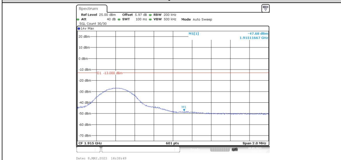
Band25-10MHz-QPSK-26640-1RB#49
