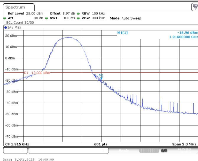
Band25-5MHz-QPSK-26665-25RB#0
