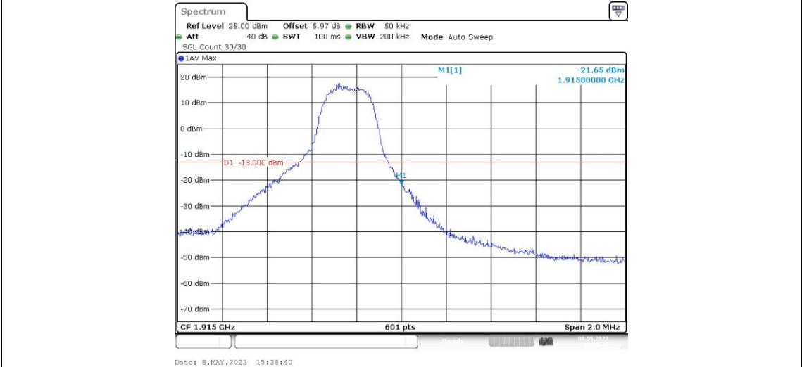
Band25-3MHz-16QAM-26675-15RB#0
