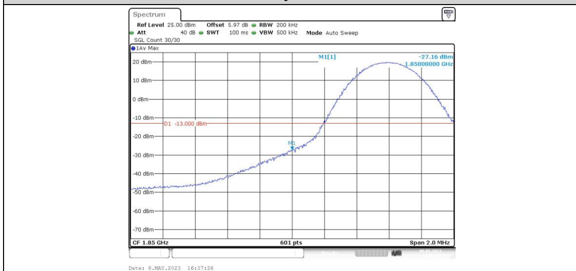
Band25-10MHz-QPSK-26090-1RB#49
