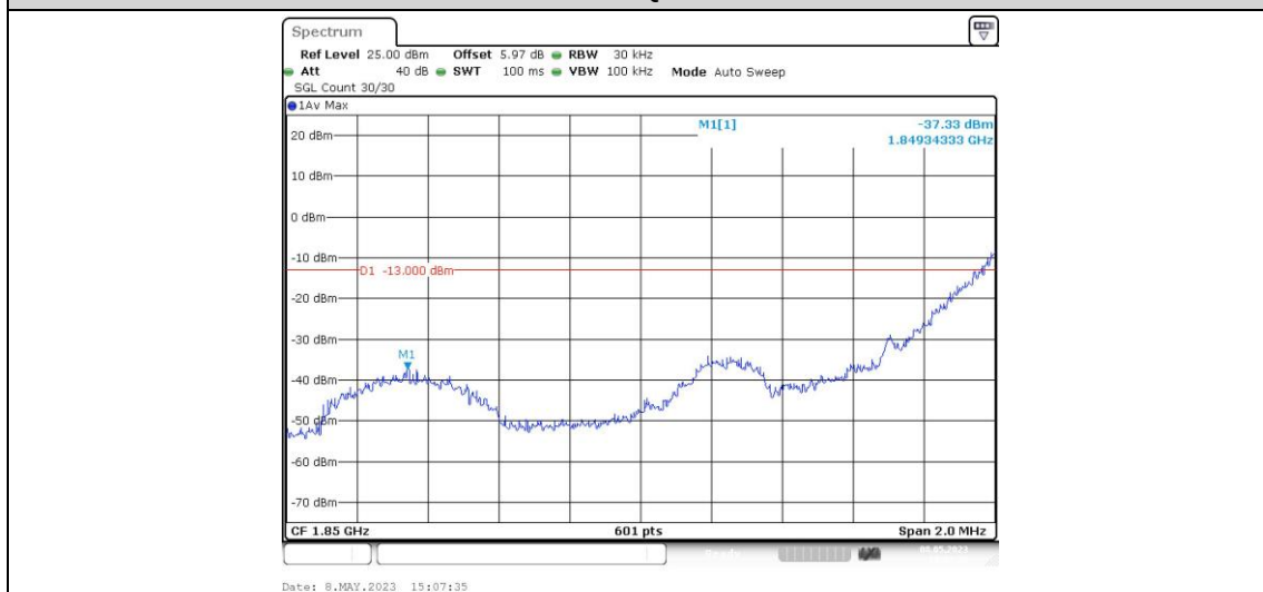
Band25-1.4MHz-16QAM-26047-6RB#0
