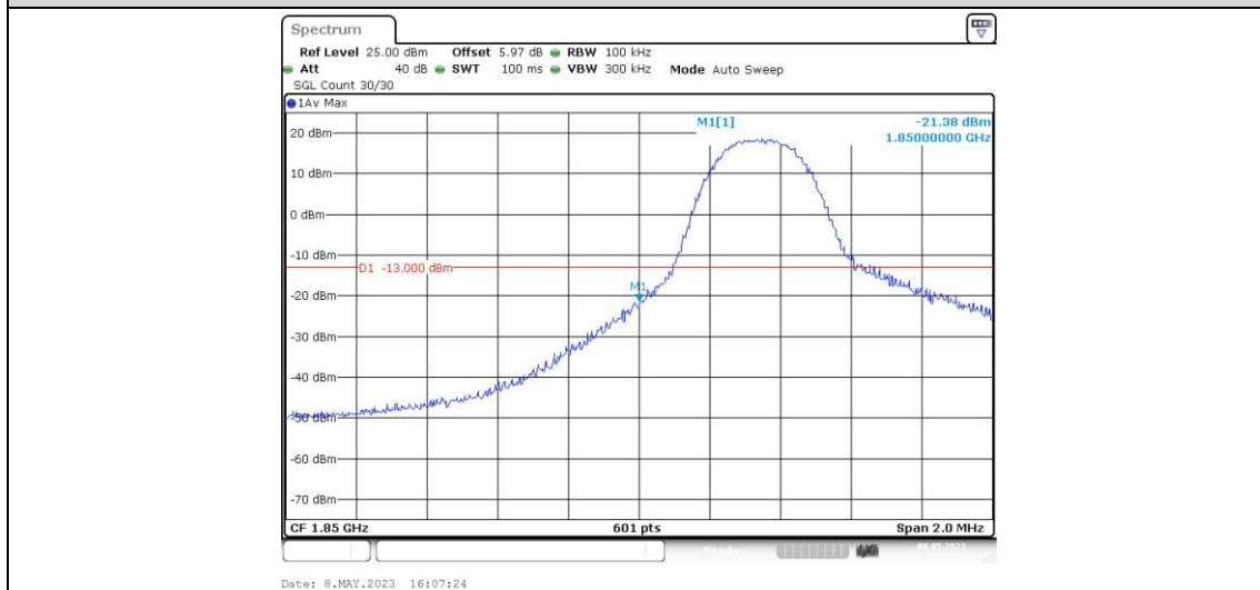
Band25-5MHz-QPSK-26065-1RB#24
