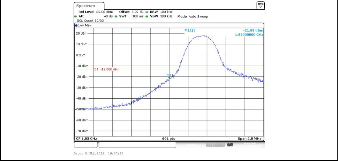
Band25-5MHz-16QAM-26065-1RB#24
