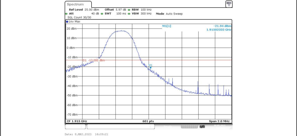
Band25-5MHz-16QAM-26665-25RB#0
