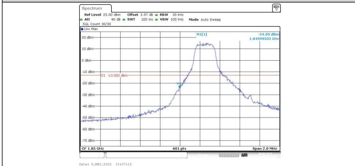
Band25-1.4MHz-16QAM-26047-1RB#5
