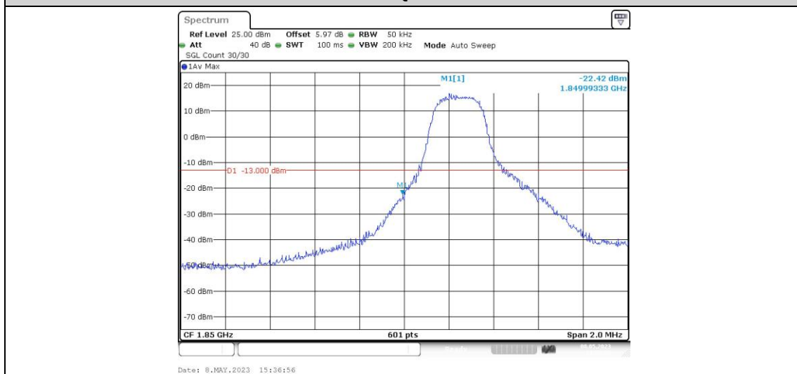
Band25-3MHz-16QAM-26055-1RB#14
