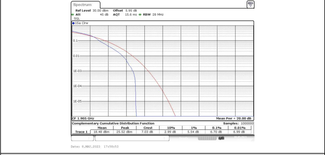
Band25-20MHz-16QAM-26590-100RB#0
