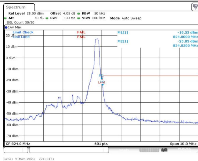
Band26-3MHz-QPSK-26775-15RB#0
