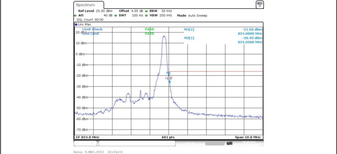
Band26-3MHz-16QAM-26775-15RB#0
