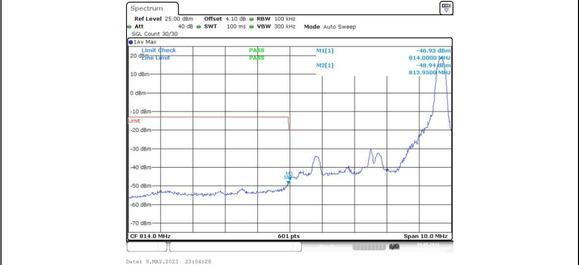
Band26-5MHz-16QAM-26715-25RB#0
