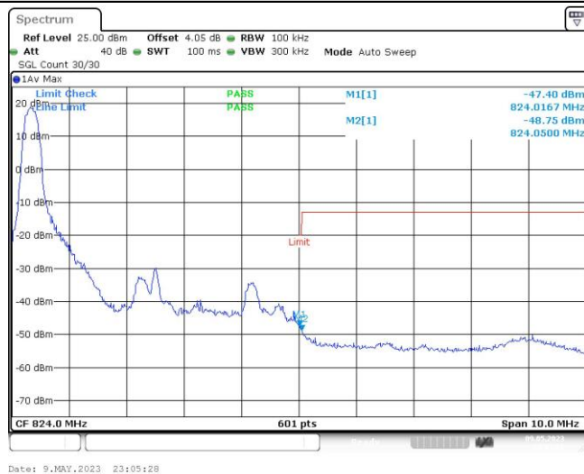
Band26-5MHz-16QAM-26765-1RB#24
