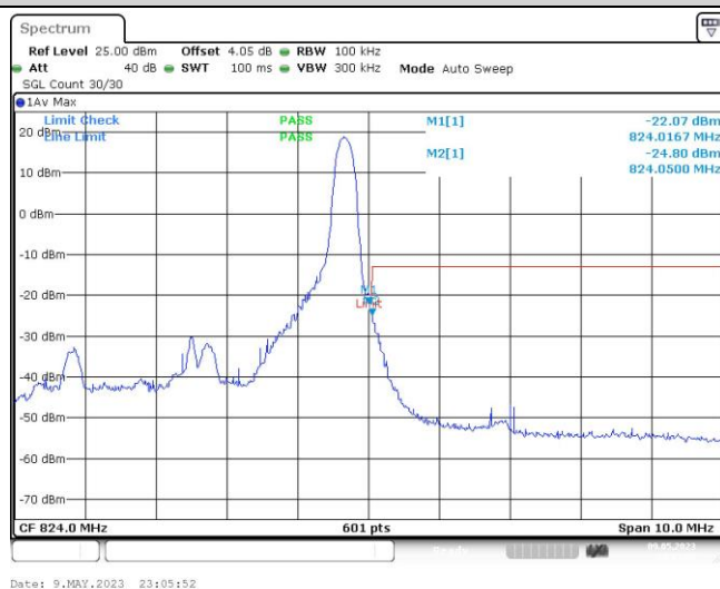
Band26-5MHz-16QAM-26765-25RB#0
