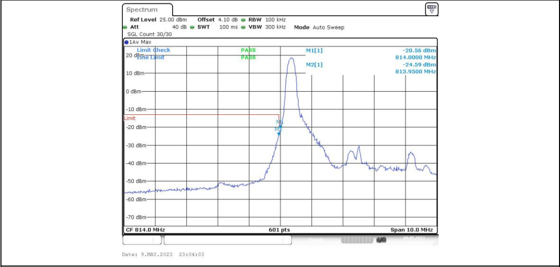
Band26-5MHz-16QAM-26715-1RB#24
