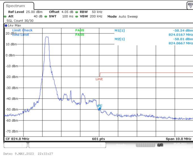
Band26-3MHz-QPSK-26775-1RB#14
