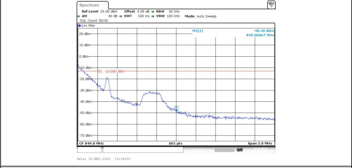
Band26-1.4MHz-16QAM-27033-1RB#5
