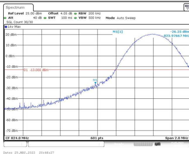
Band26-10MHz-16QAM-26840-1RB#49
