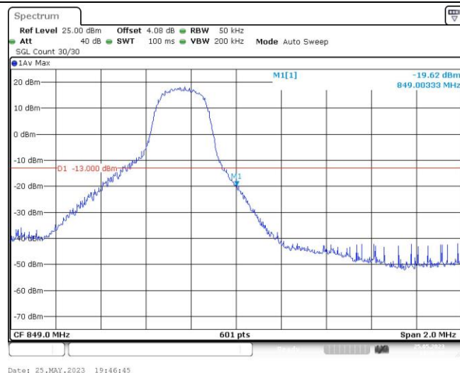
Band26-3MHz-QPSK-27025-15RB#0
