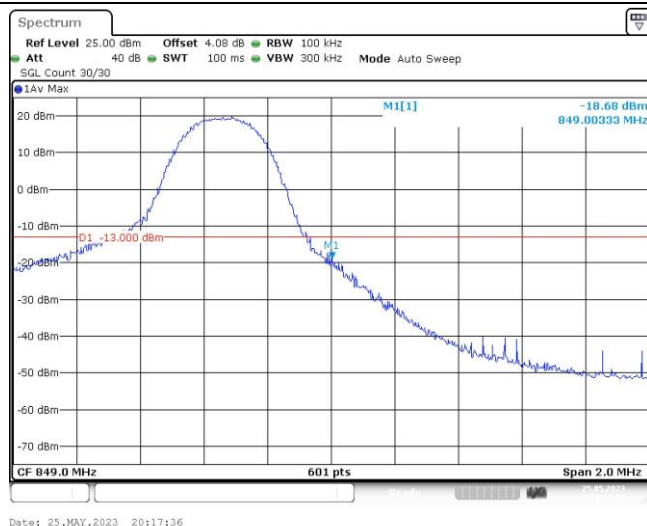
Band26-5MHz-QPSK-27015-25RB#0
