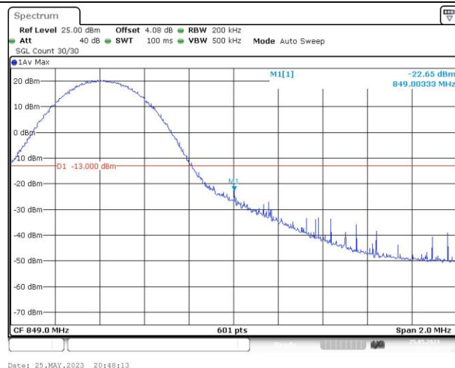
Band26-10MHz-16QAM-26990-50RB#0
