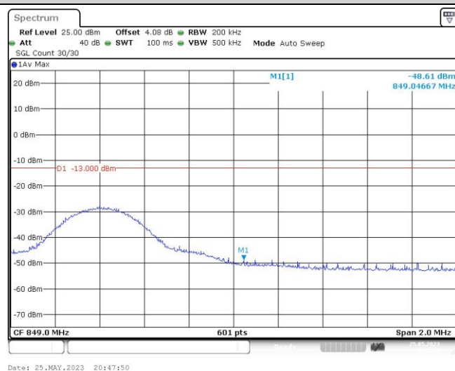
Band26-10MHz-16QAM-26990-1RB#49
