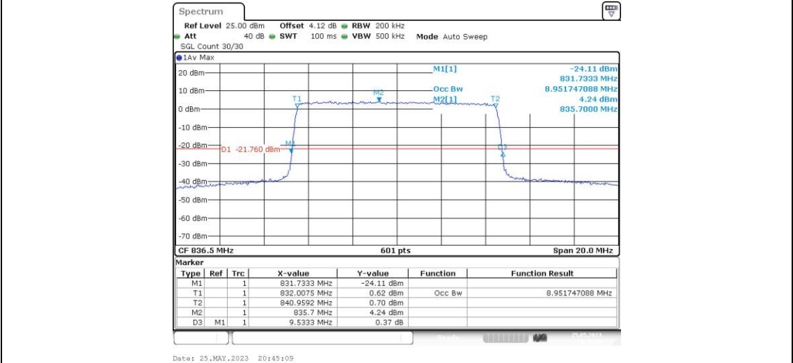
Band26-10MHz-16QAM-26990-50RB#0
