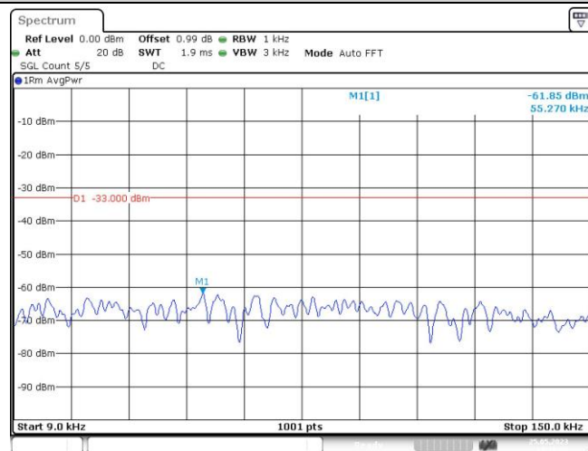
Band26-1.4MHz-QPSK-26797-1RB#0-Range1:0.009~0.15MHz
