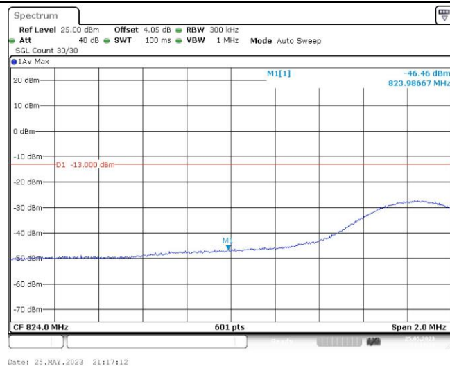
Band26-15MHz-QPSK-26865-75RB#0
