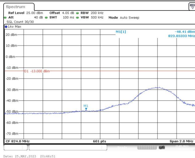
Band26-10MHz-16QAM-26840-50RB#0
