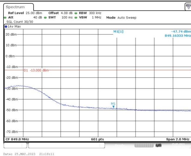
Band26-15MHz-QPSK-26965-1RB#74
