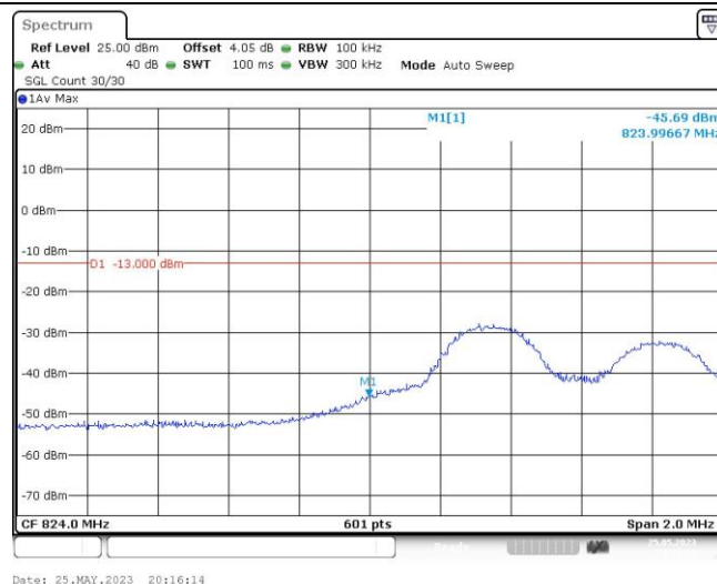
Band26-5MHz-QPSK-26815-25RB#0
