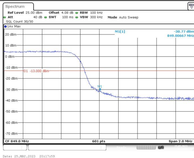
Band26-5MHz-16QAM-26815-1RB#0
