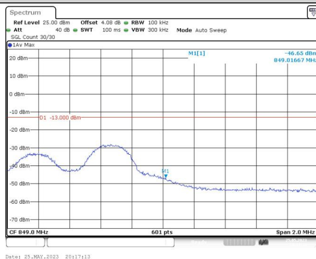
Band26-5MHz-QPSK-27015-1RB#24
