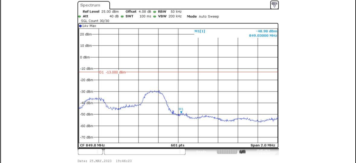
Band26-3MHz-QPSK-27025-1RB#14
