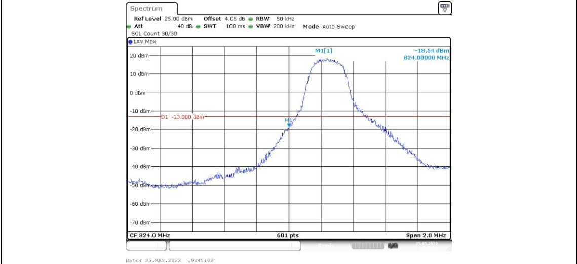
Band26-3MHz-QPSK-26805-1RB#14
