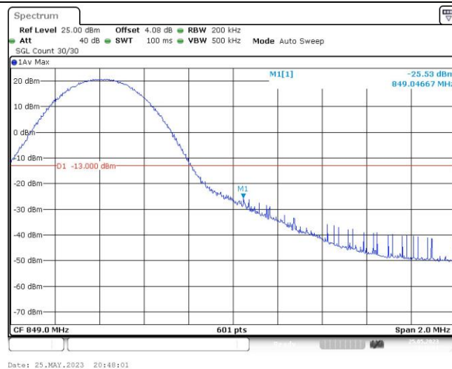
Band26-10MHz-QPSK-26990-50RB#0
