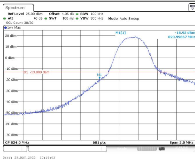
Band26-5MHz-16QAM-26815-1RB#24
