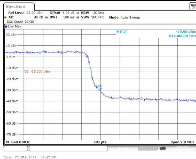
Band26-3MHz-16QAM-26805-1RB#0
