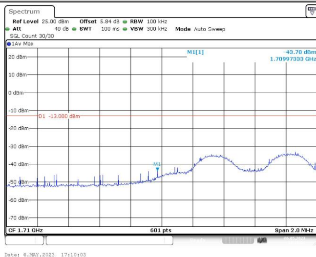
Band4-5MHz-16QAM-19975-25RB#0
