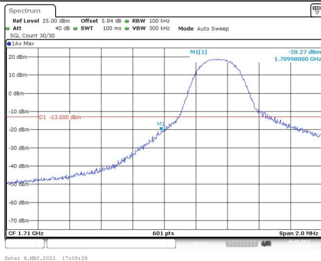
Band4-5MHz-QPSK-19975-1RB#24
