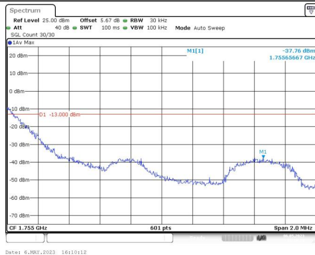
Band4-1.4MHz-16QAM-20393-1RB#5
