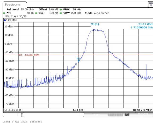
Band4-3MHz-16QAM-19965-1RB#14
