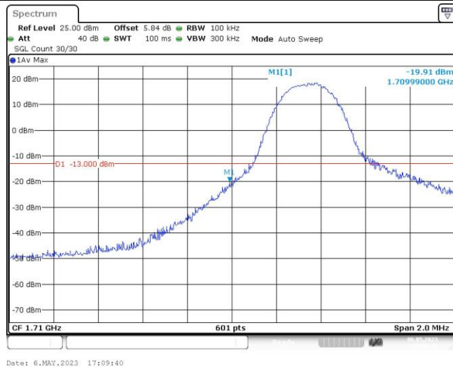
Band4-5MHz-16QAM-19975-1RB#24
