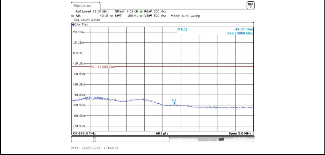
Band5-10MHz-QPSK-20600-1RB#49
