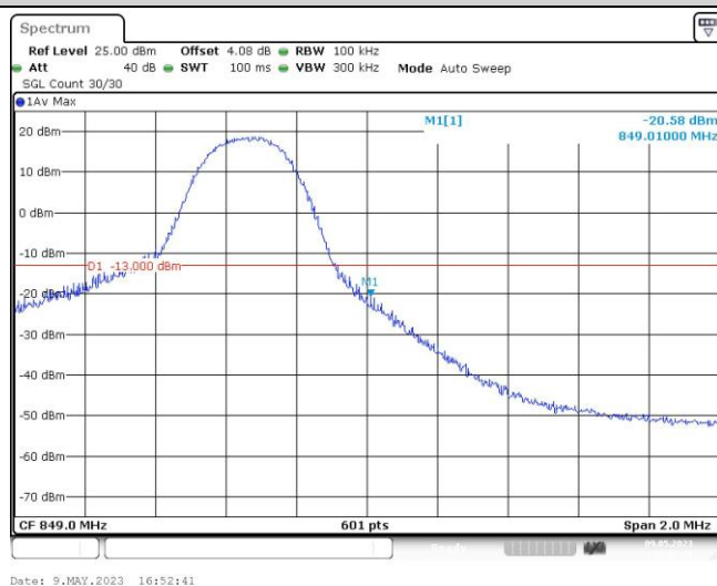
Band5-5MHz-16QAM-20625-25RB#0
