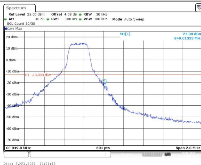
Band5-1.4MHz-16QAM-20643-6RB#0
