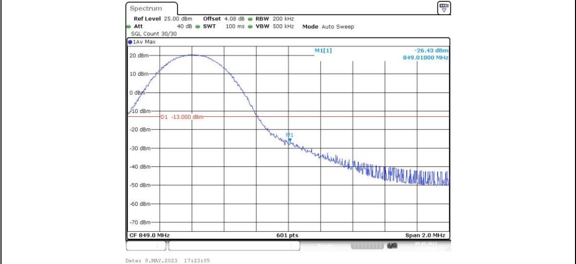
Band5-10MHz-QPSK-20600-50RB#0
