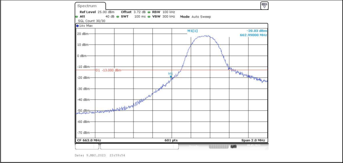
Band71-5MHz-16QAM-133147-1RB#24
