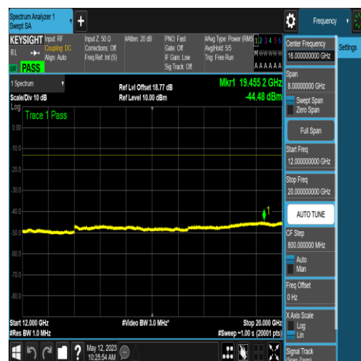
NTNV_N2_PC3_15_5_L_TID16_N/A_12000_20000_00_#1
