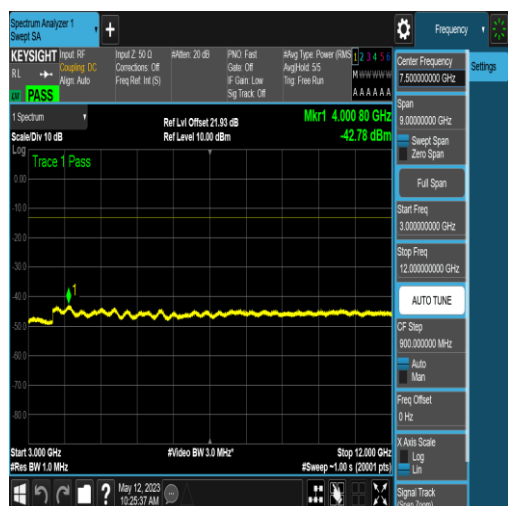
NTNV_N2_PC3_15_5_L_TID16_N/A_3000_12000_0_#1
