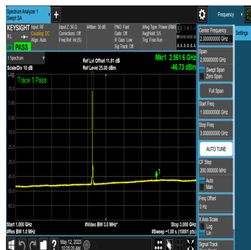
NTNV_N2_PC3_15_5_L_TID16_N/A_1000_3000_#1
