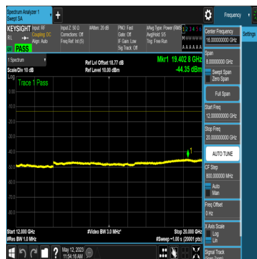
NTNV_N2_PC3_15_15_H_TID4_N/A_12000_200_00_#1
