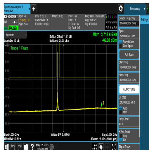
NTNV_N2_PC3_15_15_H_TID4_N/A_1000_3000_#1
