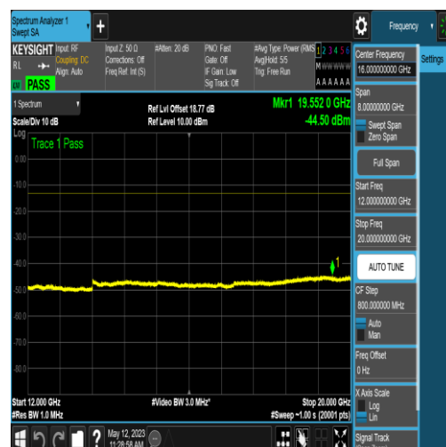
NTNV_N2_PC3_15_15_L_TID6_N/A_12000_20000_#1
