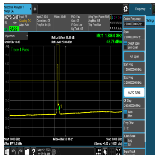
NTNV_N2_PC3_15_15_L_TID6_N/A_1000_3000_#1
