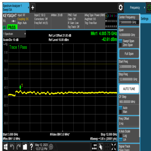
NTNV_N2_PC3_15_20_H_TID6_N/A_3000_12000_0_#1
