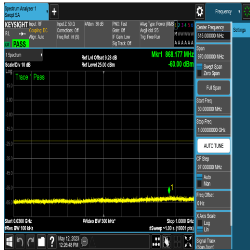
NTNV_N2_PC3_15_20_H_TID6_N/A_30_1000_#1
