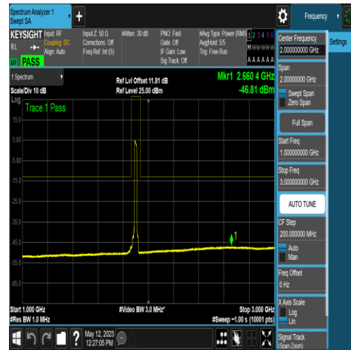
NTNV_N2_PC3_15_20_H_TID6_N/A_1000_3000_#1
