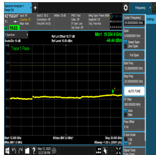
NTNV_N2_PC3_15_20_H_TID6_N/A_12000_20000_00_#1
