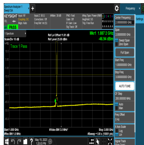
NTNV_N25_PC3_15_10_H_TID17_N/A_1000_3000_#1
