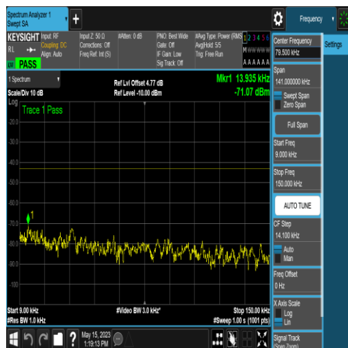
NTNV_N25_PC3_15_10_H_TID17_N/A_0.009_0. 15_#1
