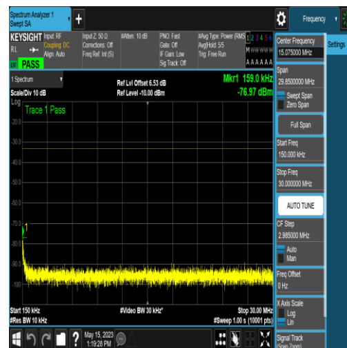
NTNV_N25_PC3_15_10_H_TID17_N/A_0.15_30_#1
