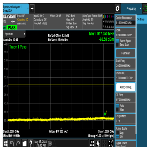
NTNV_N25_PC3_15_10_H_TID17_N/A_30_1000_#1
