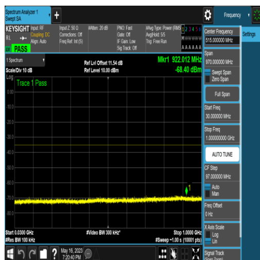
NTNV_N41_PC2_30_50_M_TID17_N/A_30_1000 _#1
