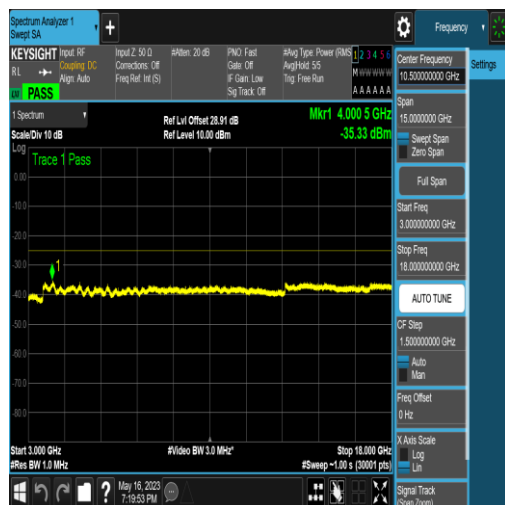
NTNV_N41_PC2_30_50_M_TID16_N/A_3000_18 000_#1
