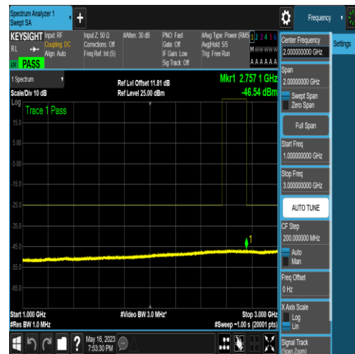
NTNV_N41_PC2_30_60_H_TID18_N/A_1000_30 00_#1
