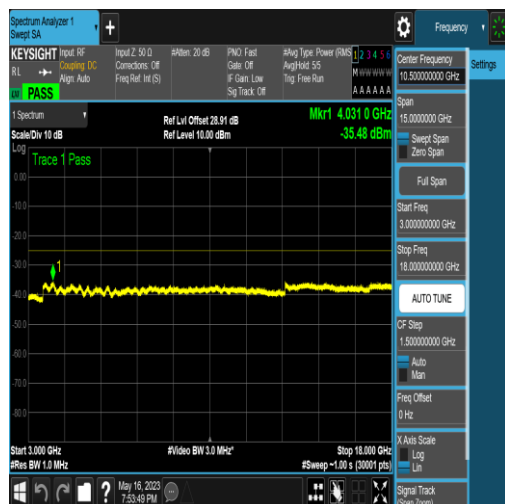
NTNV_N41_PC2_30_60_H_TID18_N/A_3000_18 000_#1
