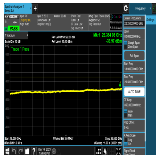
NTNV_N41_PC2_30_60_H_TID18_N/A_18000_2 6500_#1
