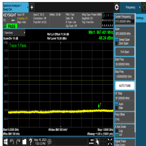
NTNV_N41_PC2_30_60_H_TID18_N/A_30_1000 _#1
