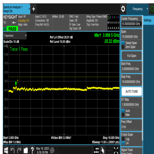
NTNV_N41_PC2_30_80_H_TID6_N/A_3000_180 00_#1
