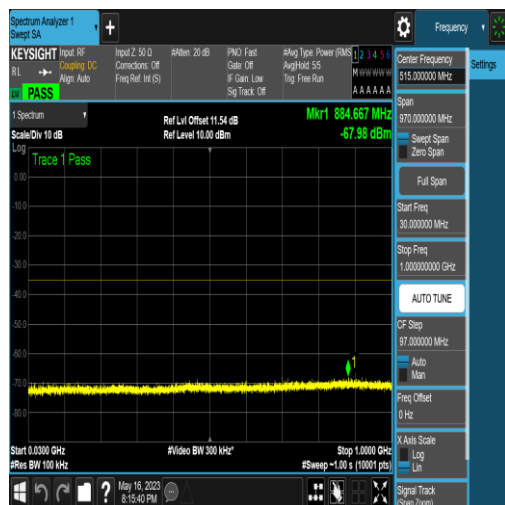
NTNV_N41_PC2_30_80_H_TID6_N/A_30_1000_ #1
