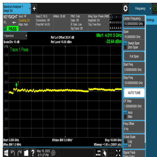
NTNV_N41_PC2_30_80_M_TID18_N/A_3000_18 000_#1
