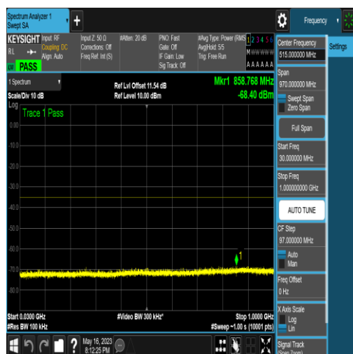
NTNV_N41_PC2_30_80_M_TID16_N/A_30_1000 _#1
