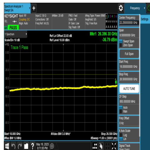
NTNV_N41_PC2_30_80_M_TID18_N/A_18000_2 6500_#1
