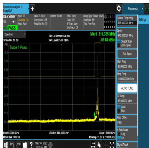
NTNV_N5_PC3_15_15_H_TID4_N/A_30_1000_#1
