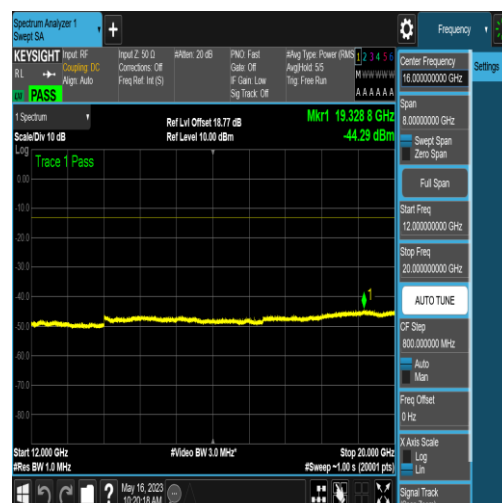
NTNV_N5_PC3_15_15_H_TID4_N/A_12000_200_00_#1
