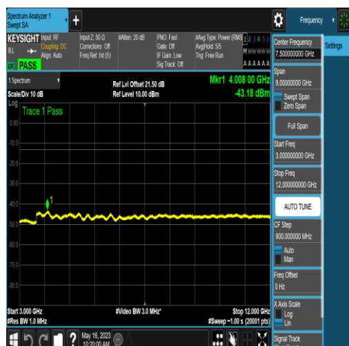
NTNV_N5_PC3_15_15_H_TID4_N/A_3000_1200_0_#1
