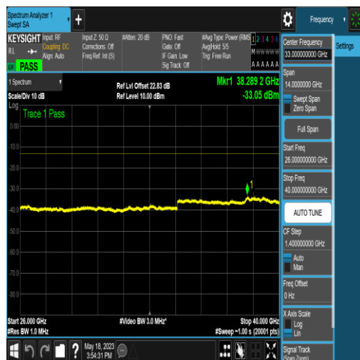
NTNV_N77-3450-3550_PC2_30_50_H_TID5_N/A _26000_40000_#1
