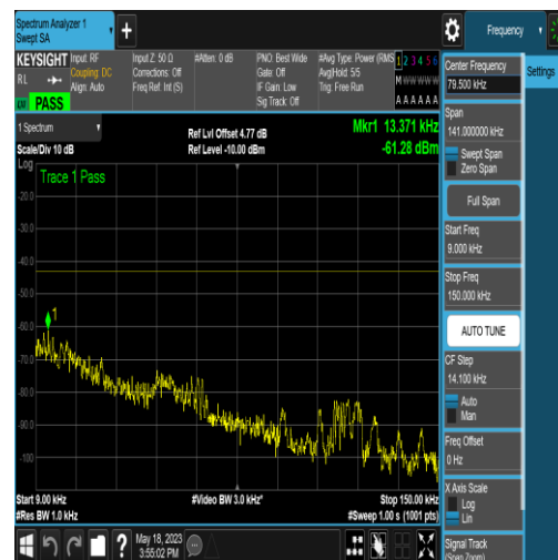
NTNV_N77-3450-3550_PC2_30_50_H_TID18_N/ A_0.009_0.15_#1
