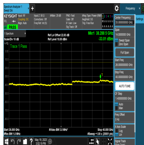
NTNV_N77-3450-3550_PC2_30_50_H_TID4_N/A _26000_40000_#1
