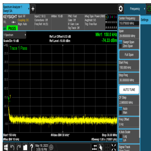
NTNV_N77-3450-3550_PC2_30_50_H_TID18_N/ A_0.15_30_#1
