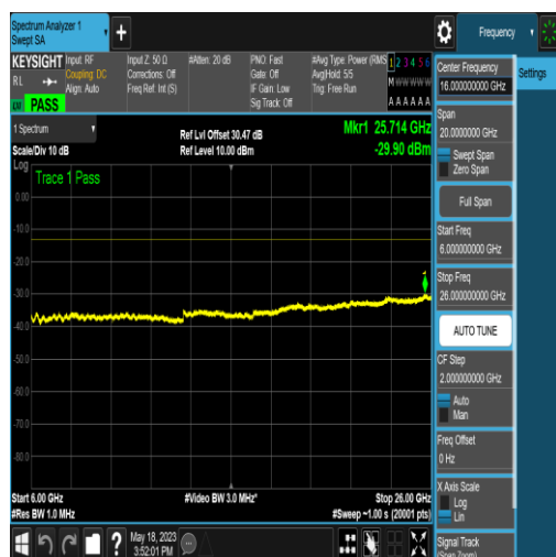
NTNV_N77-3450-3550_PC2_30_50_H_TID4_N/A _6000_26000_#1
