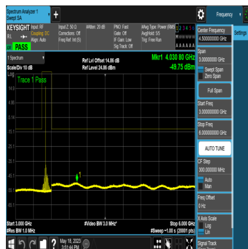
NTNV_N77-3450-3550_PC2_30_50_H_TID4_N/A _3000_6000_#1
