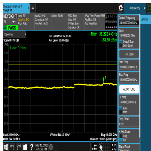
NTNV_N77-3450-3550_PC2_30_60_M_TID6_N/A _26000_40000_#1
