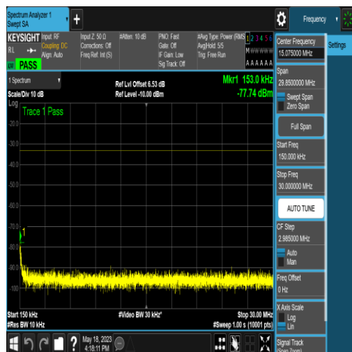
NTNV_N77-3450-3550_PC2_30_60_M_TID4_N/A _0.15_30_#1
