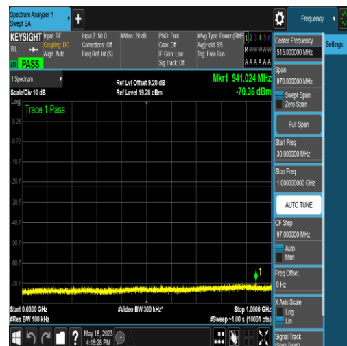
NTNV_N77-3450-3550_PC2_30_60_M_TID4_N/A _30_1000_#1
