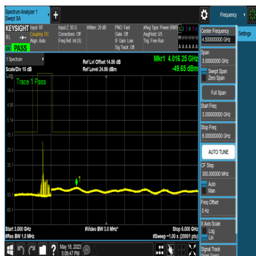
NTNV_N77-3450-3550_PC2_30_80_M_TID16_N/ A_3000_6000_#1
