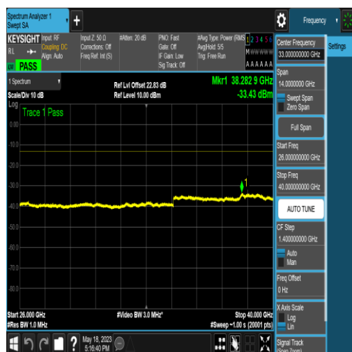
NTNV_N77-3450-3550_PC2_30_80_H_TID5_N/A _26000_40000_#1
