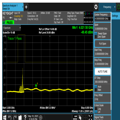
NTNV_N77-3450-3550_PC2_30_80_H_TID5_N/A _3000_6000_#1
