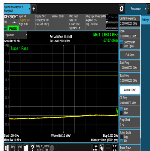
NTNV_N77-3450-3550_PC2_30_80_M_TID16_N/ A_1000_3000_#1
