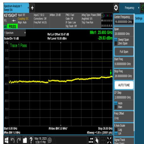
NTNV_N77-3450-3550_PC2_30_90_M_TID6_N/A _6000_26000_#1
