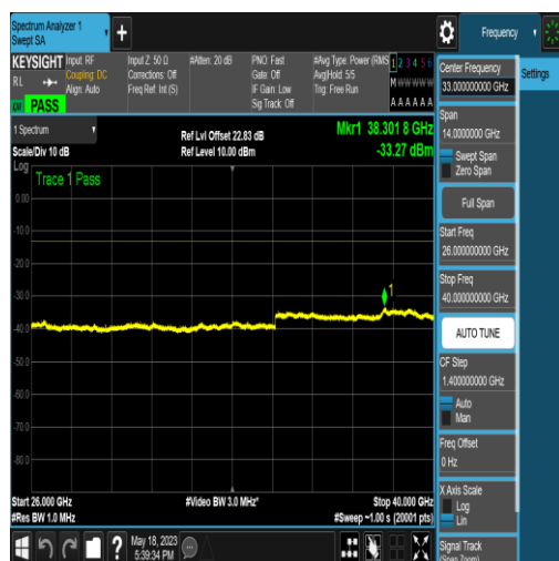
NTNV_N77-3450-3550_PC2_30_90_M_TID6_N/A _26000_40000_#1
