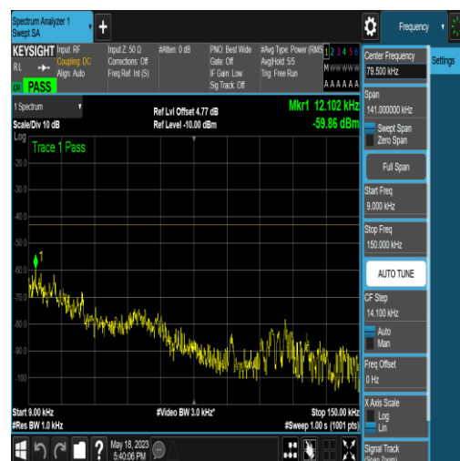
NTNV_N77-3450-3550_PC2_30_90_M_TID4_N/A _0.009_0.15_#1
