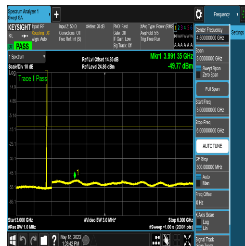
NTNV_N77-3450-3550_PC2_30_10_M_TID17_N/ A_3000_6000_#1
