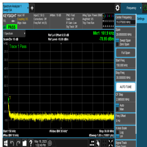
NTNV_N77-3450-3550_PC2_30_10_M_TID17_N/ A_0.15_30_#1
