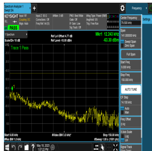
NTNV_N77-3450-3550_PC2_30_10_H_TID4_N/A _0.009_0.15_#1
