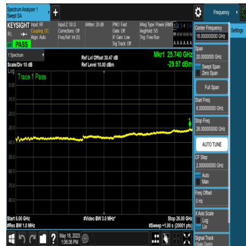
NTNV_N77-3450-3550_PC2_30_10_H_TID6_N/A _6000_26000_#1
