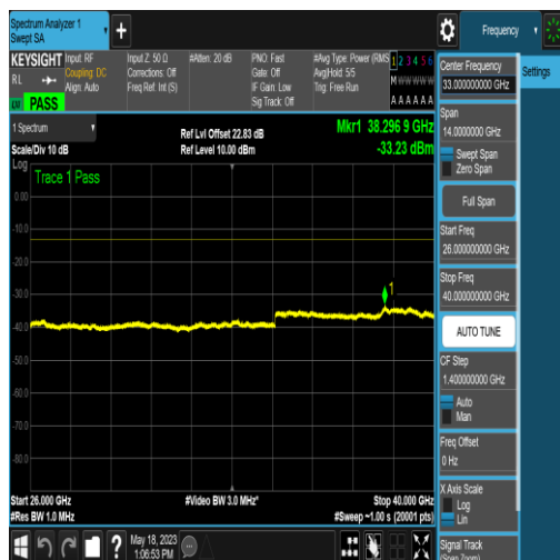
NTNV_N77-3450-3550_PC2_30_10_H_TID6_N/A _26000_40000_#1
