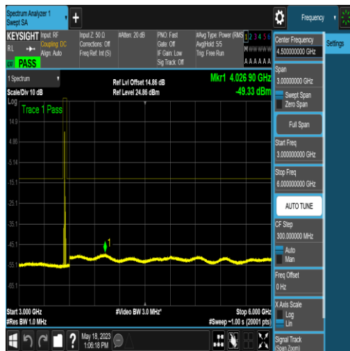
NTNV_N77-3450-3550_PC2_30_10_H_TID6_N/A _3000_6000_#1
