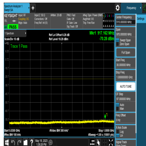
NTNV_N77-3450-3550_PC2_30_15_M_TID18_N/ A_30_1000_#1
