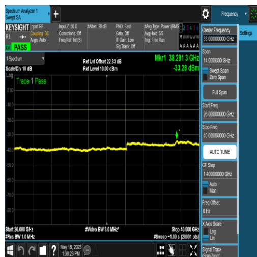
NTNV_N77-3450-3550_PC2_30_15_M_TID5_N/A _26000_40000_#1
