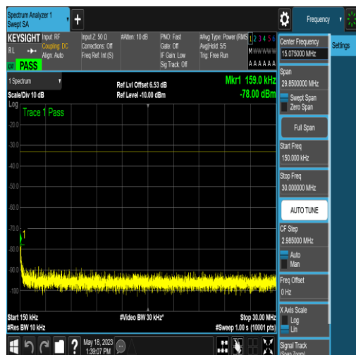
NTNV_N77-3450-3550_PC2_30_15_M_TID18_N/ A_0.15_30_#1
