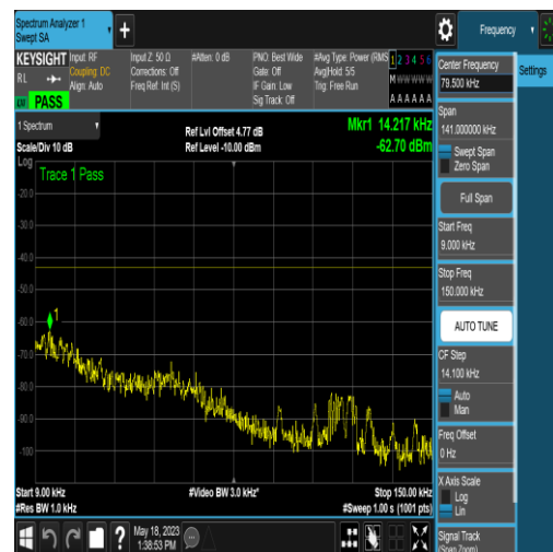
NTNV_N77-3450-3550_PC2_30_15_M_TID18_N/ A_0.009_0.15_#1
