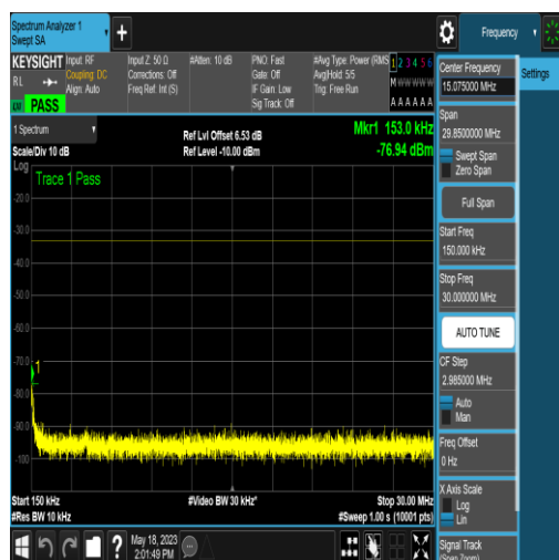
NTNV_N77-3450-3550_PC2_30_20_L_TID4_N/A _0.15_30_#1
