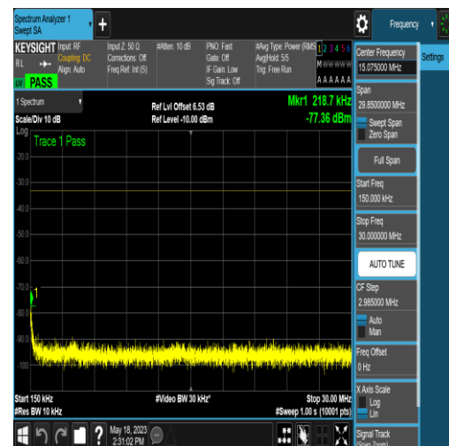
NTNV_N77-3450-3550_PC2_30_20_H_TID5_N/A _0.15_30_#1
