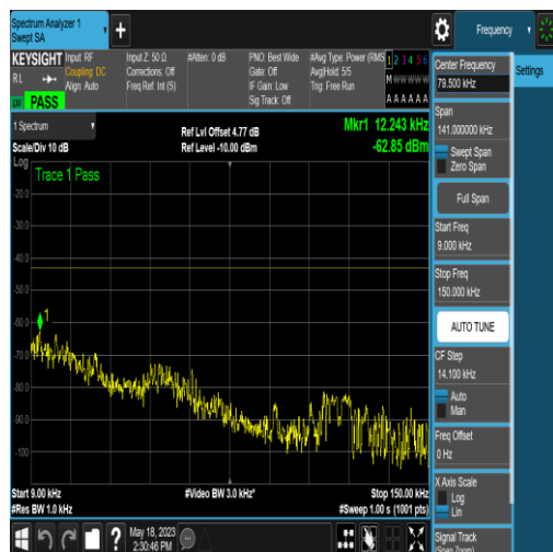
NTNV_N77-3450-3550_PC2_30_20_H_TID5_N/A _0.009_0.15_#1
