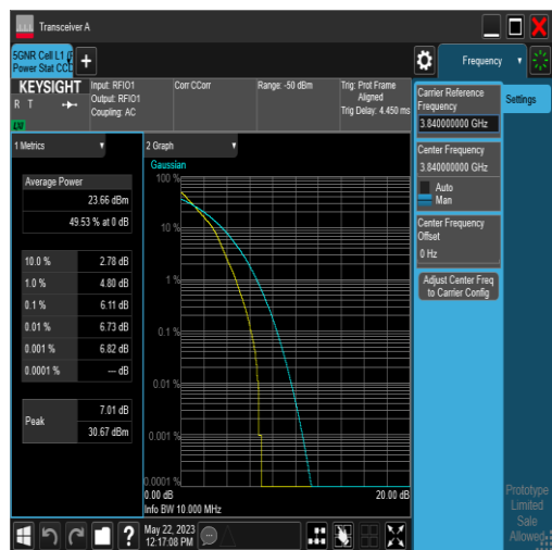
NTNV_N77-3700-3980_PC2_30_10_M_TID2_#1
