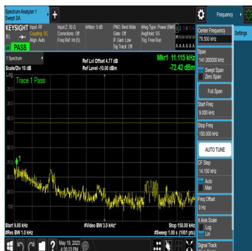
NTNV_N77-3700-3980_PC2_30_40_M_TID5_NS _01_0.009_0.15_#1
