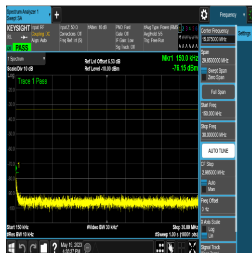
NTNV_N77-3700-3980_PC2_30_40_M_TID5_NS _01_0.15_30_#1
