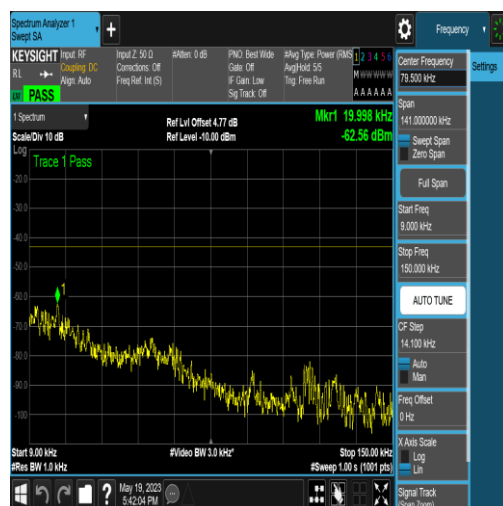
NTNV_N77-3700-3980_PC2_30_60_L_TID4_NS_ 01_0.009_0.15_#1
