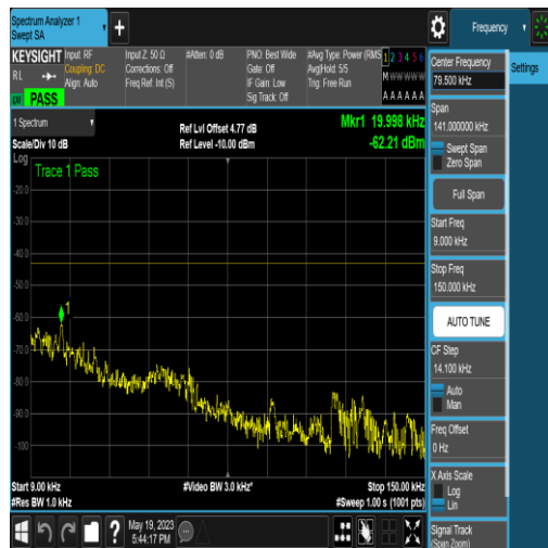
NTNV_N77-3700-3980_PC2_30_60_L_TID5_NS_ 01_0.009_0.15_#1
