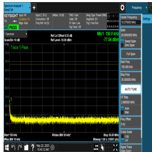
NTNV_N77-3700-3980_PC2_30_80_L_TID16_NS _01_0.15_30_#1
