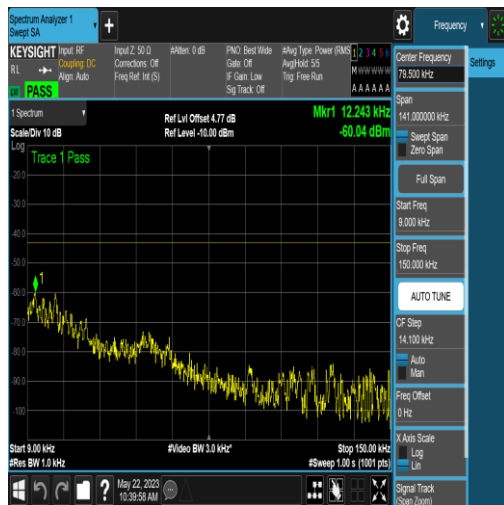
NTNV_N77-3700-3980_PC2_30_80_L_TID16_NS _01_0.009_0.15_#1
