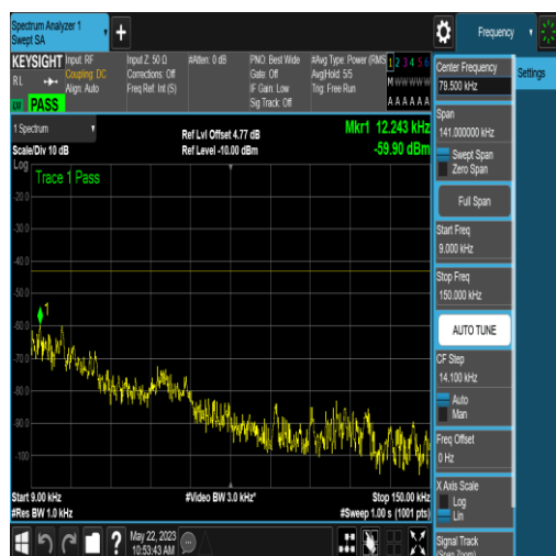
NTNV_N77-3700-3980_PC2_30_80_M_TID16_N S_01_0.009_0.15_#1
