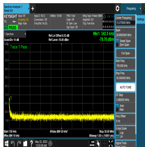
NTNV_N77-3700-3980_PC2_30_80_M_TID16_N S_01_0.15_30_#1
