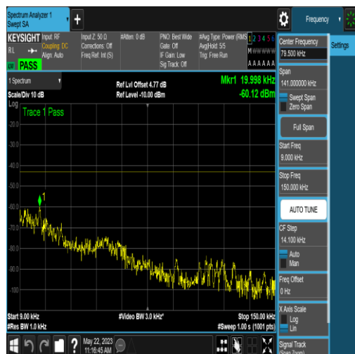
NTNV_N77-3700-3980_PC2_30_90_L_TID5_NS_ 01_0.009_0.15_#1
