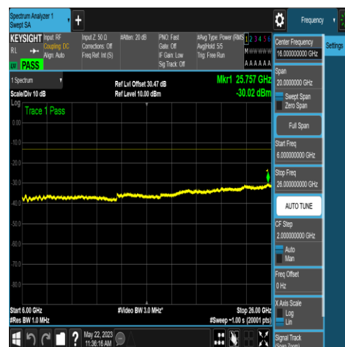
NTNV_N77-3700-3980_PC2_30_90_M_TID16_N S_01_6000_26000_#1
