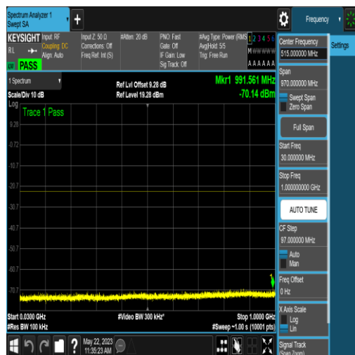
NTNV_N77-3700-3980_PC2_30_90_M_TID16_N S_01_30_1000_#1
