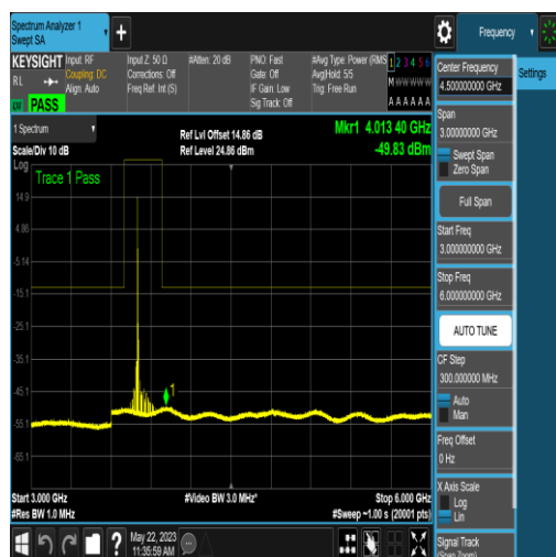
NTNV_N77-3700-3980_PC2_30_90_M_TID16_N S_01_3000_6000_#1
