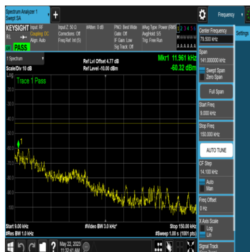
NTNV_N77-3700-3980_PC2_30_90_M_TID18_N S_01_0.009_0.15_#1
