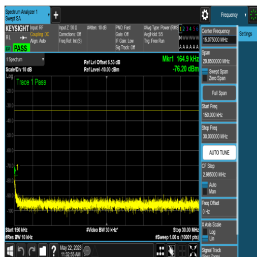
NTNV_N77-3700-3980_PC2_30_90_M_TID18_N S_01_0.15_30_#1
