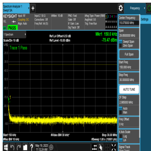
NTNV_N77-3700-3980_PC2_30_100_L_TID18_N S_01_0.15_30_#1
