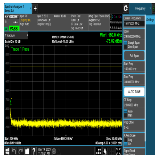
NTNV_N77-3700-3980_PC2_30_100_M_TID6_N S_01_0.15_30_#1
