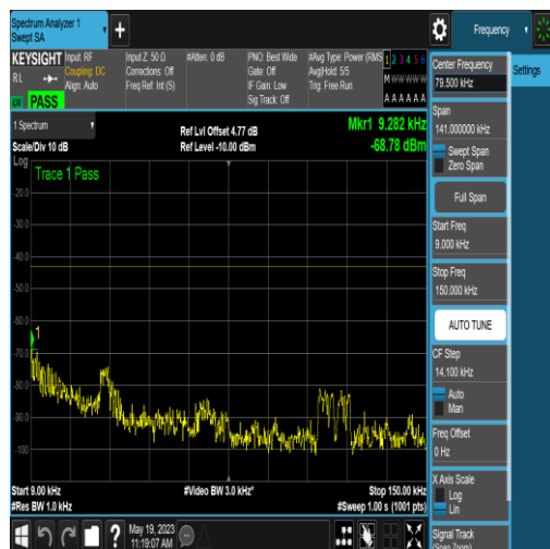
NTNV_N77-3700-3980_PC2_30_100_M_TID6_N S_01_0.009_0.15_#1
