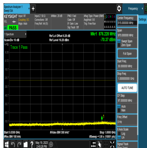
NTNV_N77-3700-3980_PC2_30_10_H_TID18_N S_01_30_1000_#1
