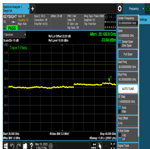
NTNV_N77-3700-3980_PC2_30_10_H_TID5_NS _01_26000_40000_#1
