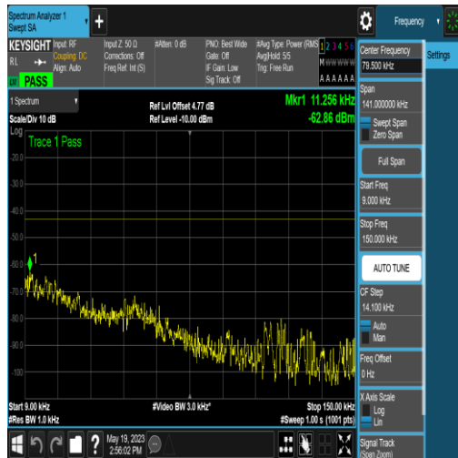
NTNV_N77-3700-3980_PC2_30_15_L_TID16_NS _01_0.009_0.15_#1
