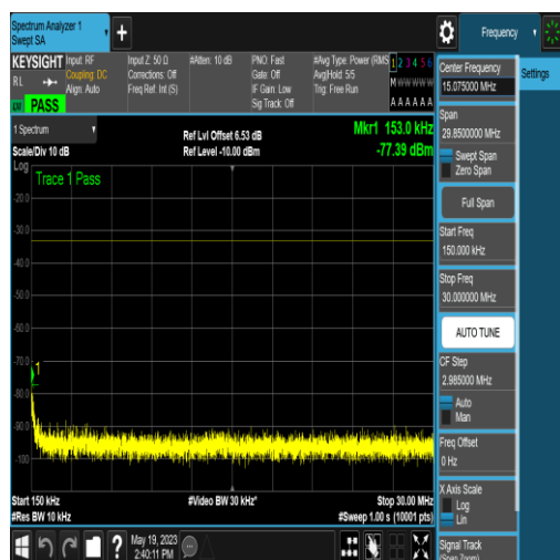
NTNV_N77-3700-3980_PC2_30_10_H_TID18_N S_01_0.15_30_#1
