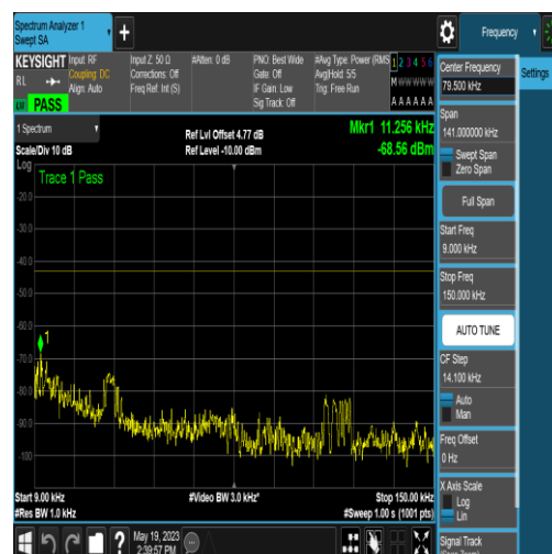
NTNV_N77-3700-3980_PC2_30_10_H_TID18_N S_01_0.009_0.15_#1
