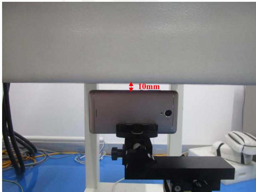
Body Right Setup Photo
