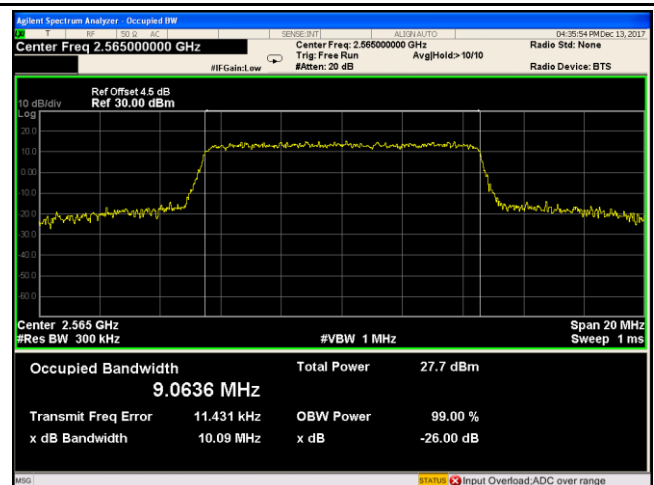
LTE Band VII - High CH 16QAM-10
