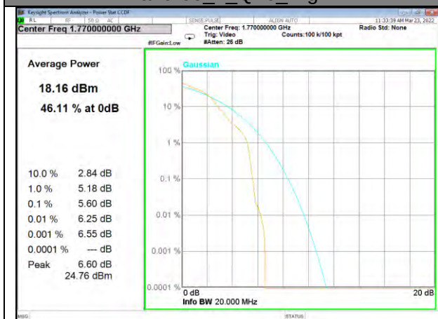
Band 66_1_Q16_High
