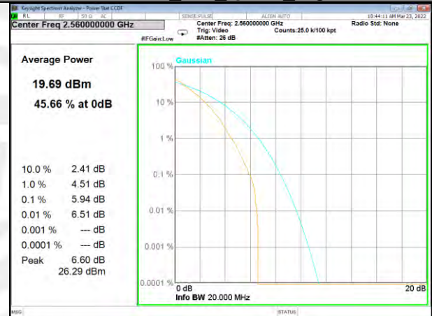
Band 7_100_Q16_High
