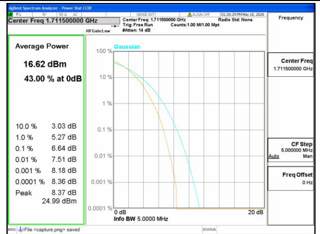
B4 / 3MHz / Low CH / 256QAM
