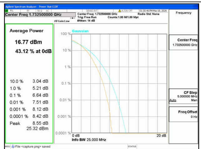
B4 / 15MHz / Mid CH / 256QAM
