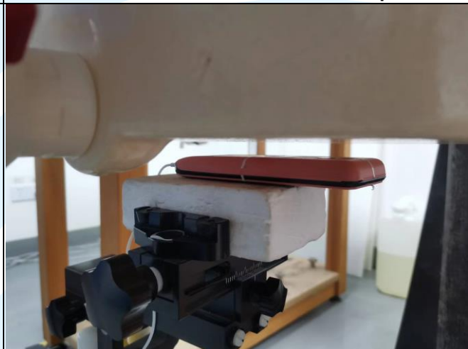
Rear Face of EUT with 1.0 cm Gap (Headset)
