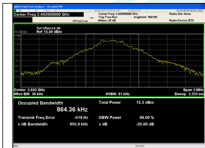
GFSK DH5 Channel 0
