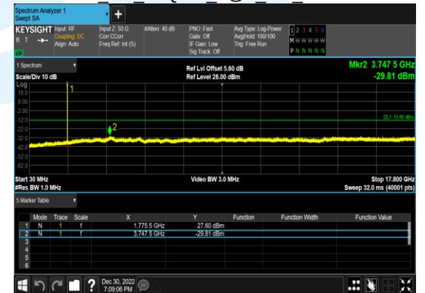
B66 5M 64QAM 1@0 CH 132647
