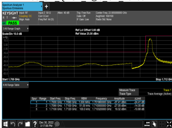
B66 5M 16QAM 1@0 CH 131997
