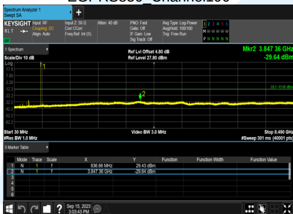
EGPRS850 Channel190
