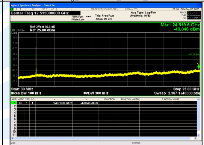
Spurious Emission IEEE 802.11g Channel 11 20MHz Antenna 0
