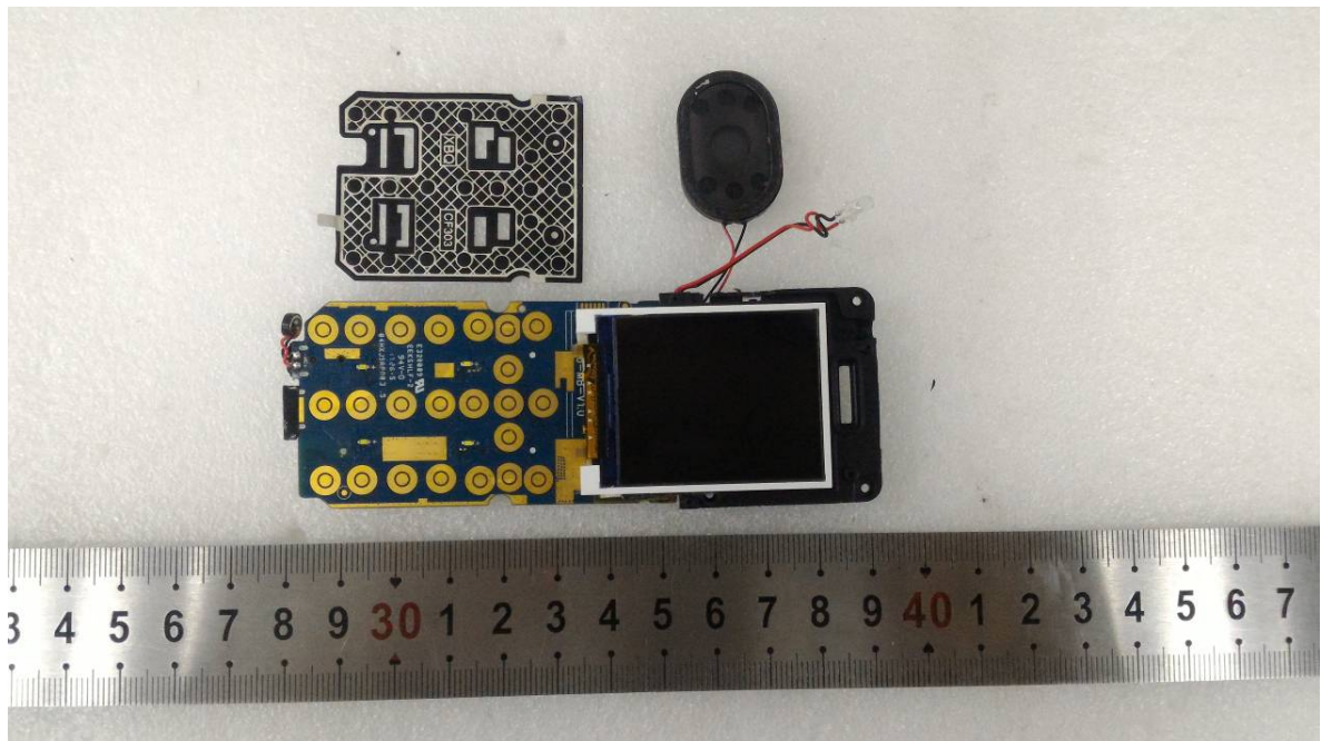
EUT – Mainboard Bottom Cover off View 1
