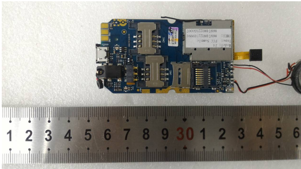
EUT – Mainboard Top View 2
