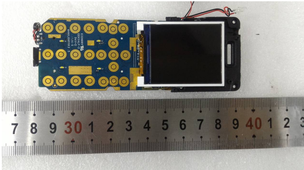
EUT – Mainboard Bottom Cover off View 2
